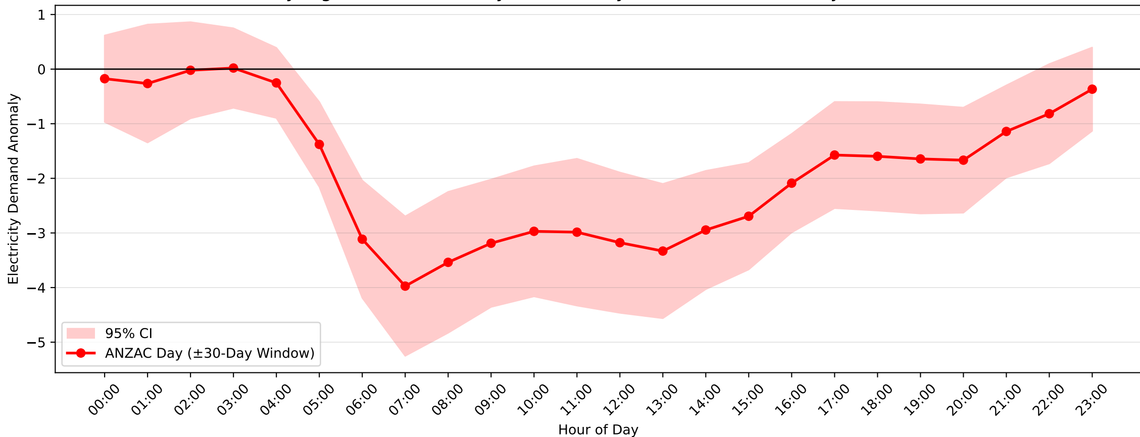
Wyong Demand Anomaly: ANZAC Day (2004-2017, \pm 30 -Day Window)
